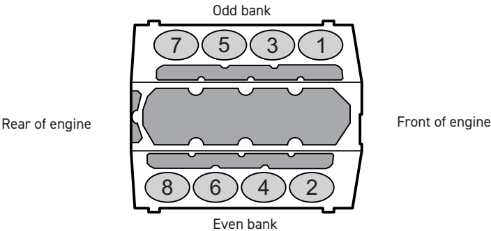
Cylinder numbers of a GM LS engine
