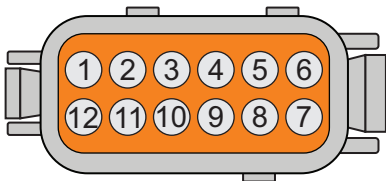
Main harness side view
